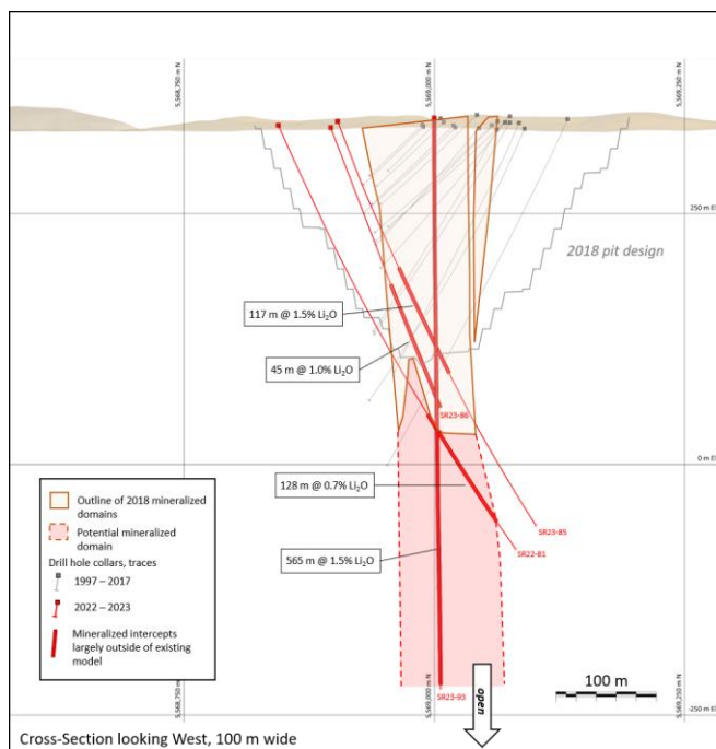
Figure 2: West-East Long Section, Separation Rapids Lithium Deposit
